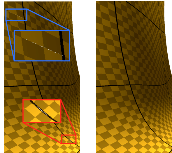
Figure 4: Crack Artifacts. Cracks – highlighted with boxes – occur during curve-based sub-patch reconstruction. Tensor product blossoms (right) are crack free. Black curves mark base-patch borders.
