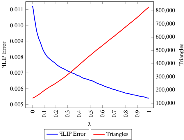
Figure 6: Changes in LIP error and triangle count with varying \lambda . For the first camera perspective in Tab. 1, we use a fixed \epsilon = 1 . Note that a larger \lambda shifts the sensitivity of our error metric to the parametrization quality required for accurate texture mapping. As intended, more triangles are generated, and the LIP error relative to the ground truth decreases.
